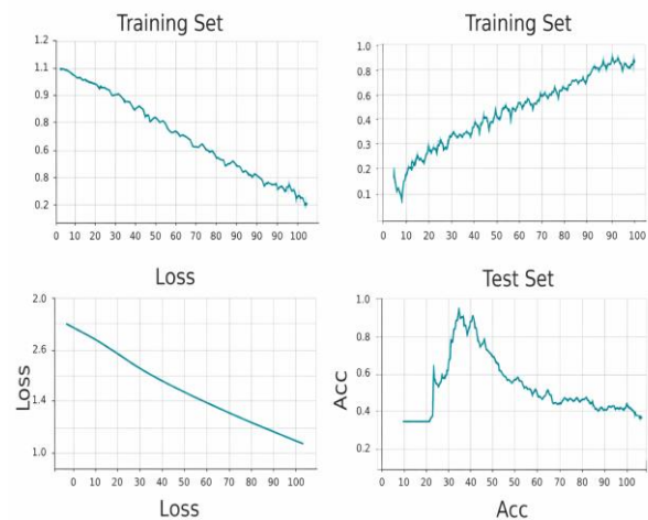
Figure 3. CNN Model Accuracy and Loss During Training.
